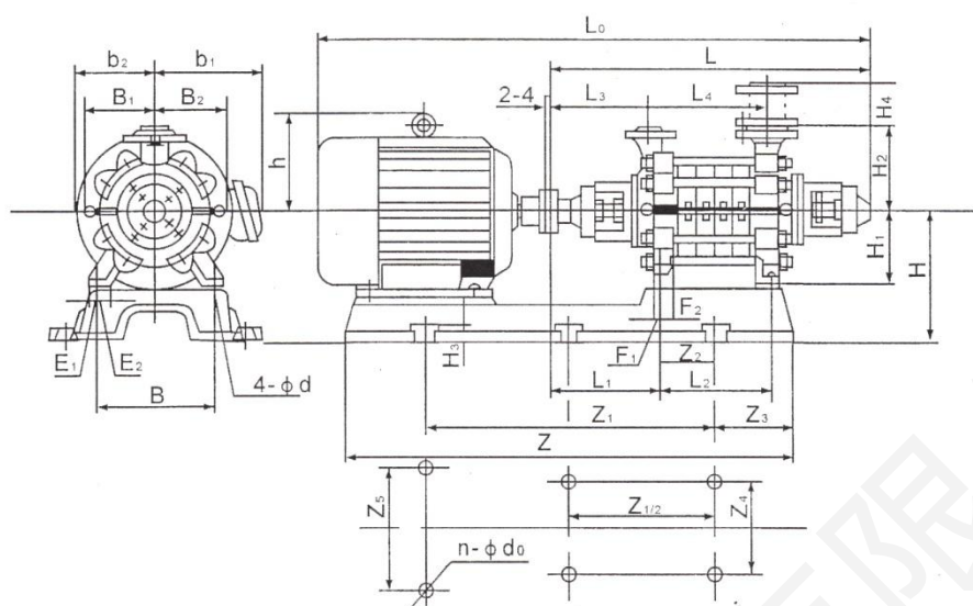
外形安装尺寸图 Overall and Installation Dimention
